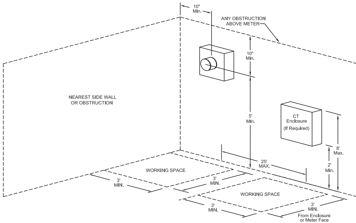
PREFERRED INSTALLATION METER SOCKET & CT ENCLOSURE MINIMUM CLEARANCES
