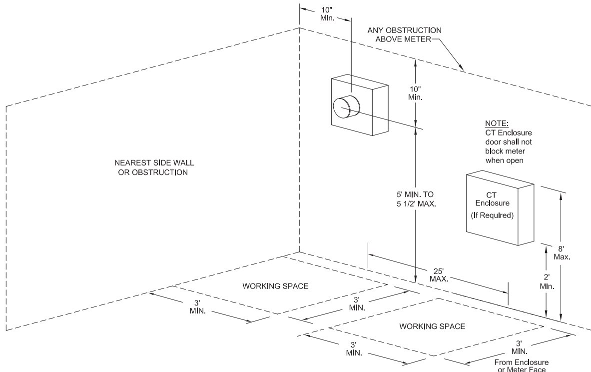
METER SOCKET & CT ENCLOSURE MINIMUM CLEARANCES
