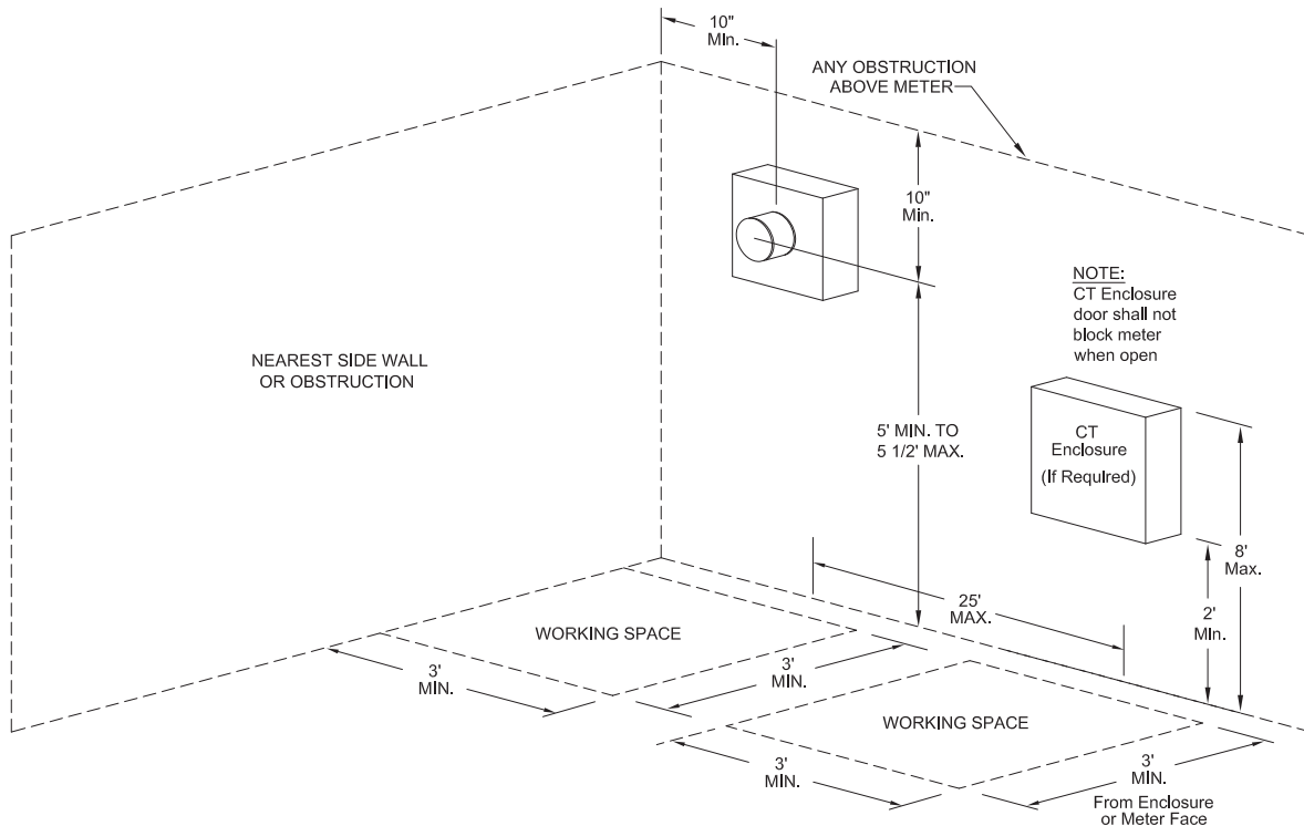
METER SOCKET & CT ENCLOSURE MINIMUM CLEARANCES
